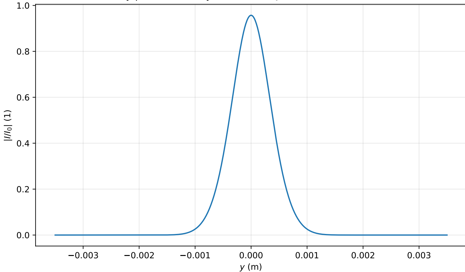
Intensity profile I(x=0, y, z=0.876)/I_0 , P_{in}=0.3P_{cr} , artificial time
